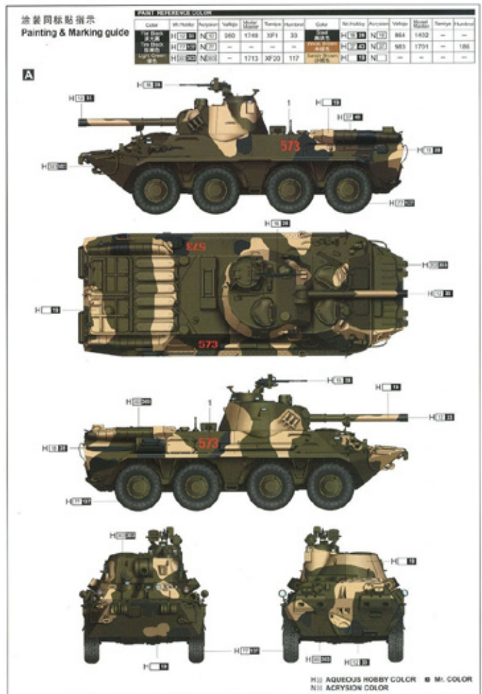
09559 1/35 2S23 Self-propelled Howitzer
